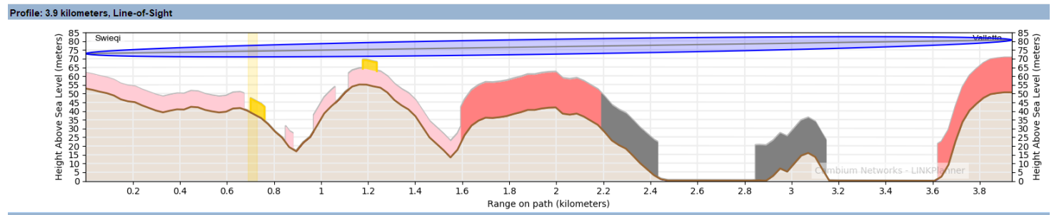
Path profile with clutter and obstructions.
